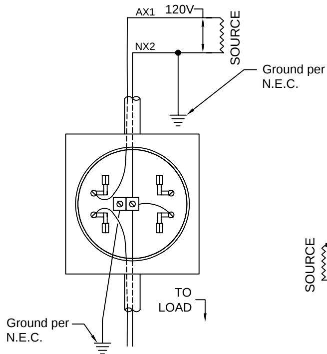
TYPE S 2 WIRE SINGLE PHASE 120 VOLTS
